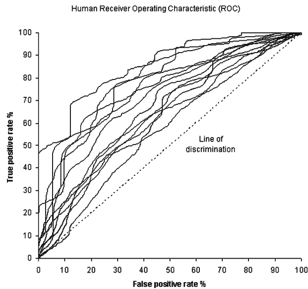
Fig. 10. Receiver operating characteristic (ROC) curves for 12 human participants with variability in the P3 detection criteria. Note, true negative rate and false negative rate do not need to be plotted, as they are fully defined by the true positive and false positive rate (respectively), e.g. true negative rate + false positive rate = 100%
